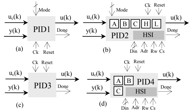
Fig. 2. Various PID IP-cores. (a) commercial PID with constant coefficients; (b) commercial PID with time varying coefficients; (c) incremental PID with constant coefficients; (d) incremental PID with time varying coefficients;
